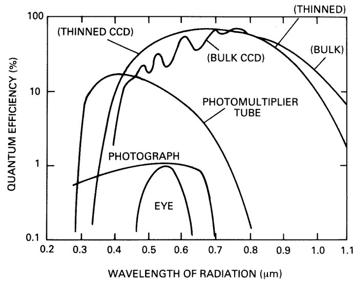
Figure 3: The sensitivity or quantum efficiency as a function of wavelength for various types of detectors. The quantum efficiency is simply the fraction of incident photons which are detected. Here it is plotted on a logarithmic scale. Thinned and bulk CCDs are simply different types of CCDs. Photomultiplier tubes are used in photoelectric photometers. Note that CCDs are more sensitive to red light than photomultiplier tubes. Adapted from McLean[56]
