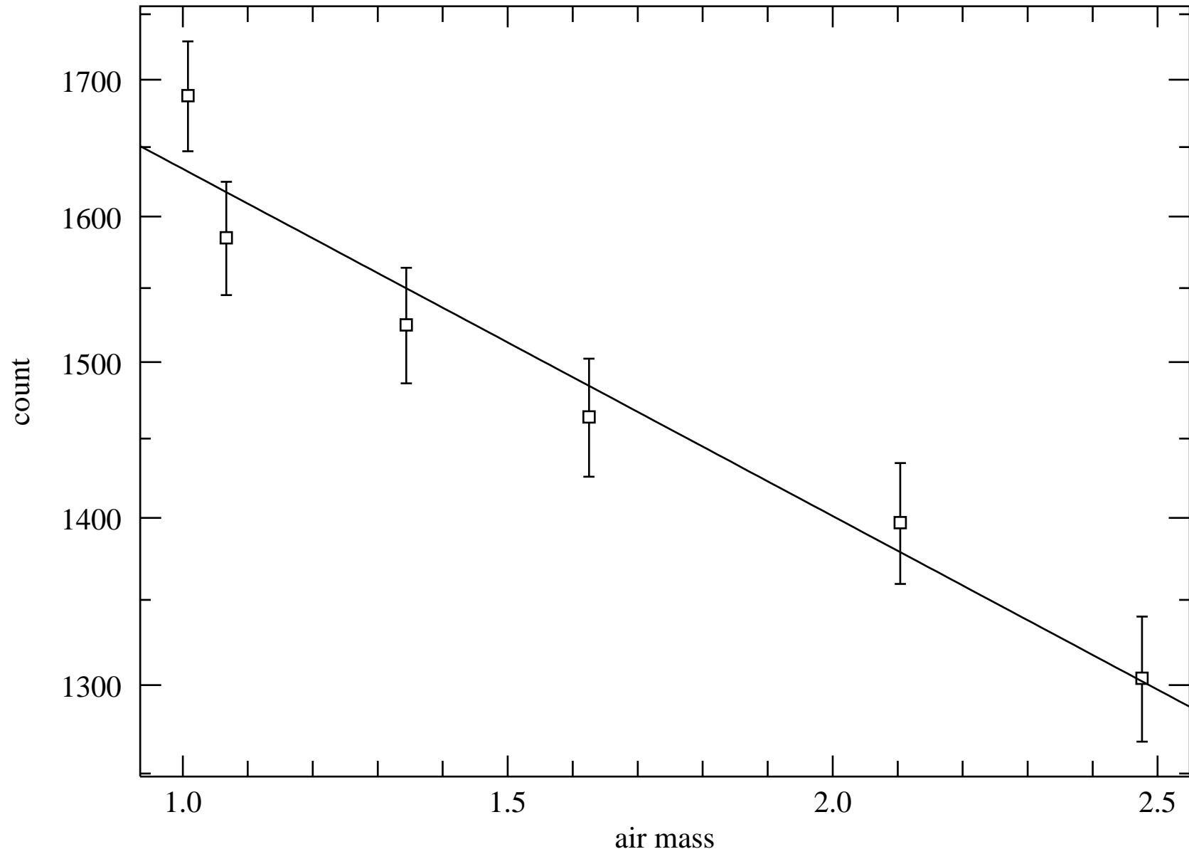
tau problem
